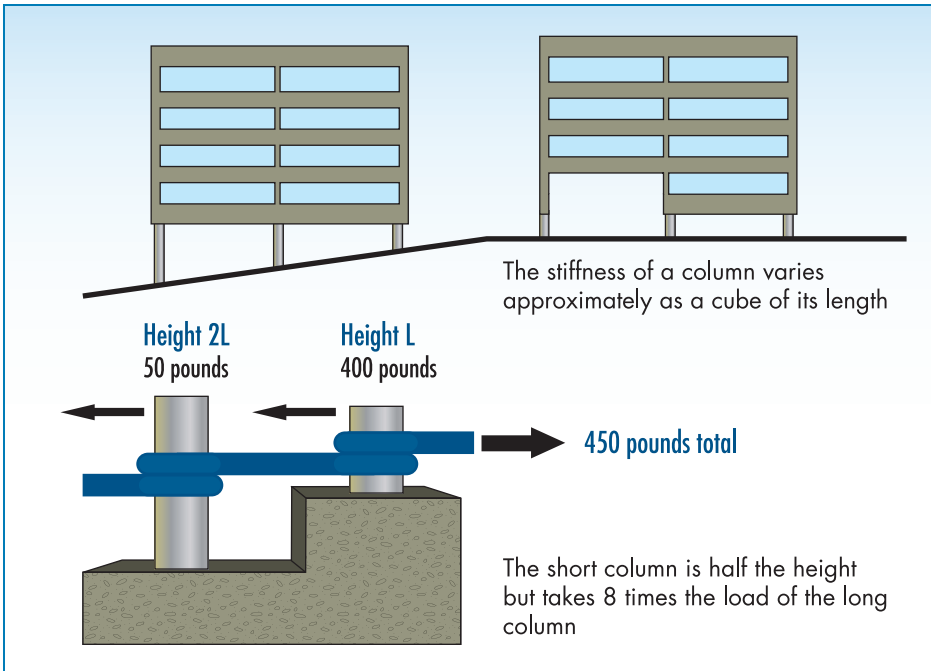
Figure 2-8: The short column problem
