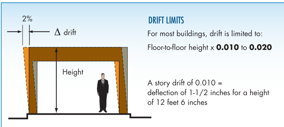
Figure 2-9: Allowable story drift
